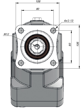
PISTON PUMP
